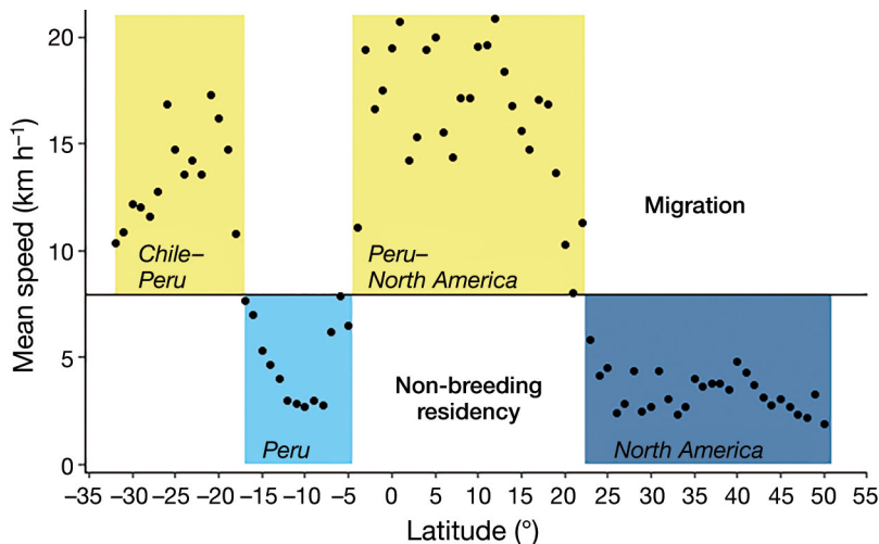
Fig. 2. Mean speed in 1° latitude bins of tracked pink-footed shearwaters Ardeana creatopus across their non-breeding-season range (32°S–51°N). Horizontal black line indicates median value used to determine migratory corridor (>median) vs. non-breeding residency (<median) areas. Migratory corridors between Chilean breeding range and Peru, and between Peru and North America, are highlighted in yellow. Non-breeding residency areas off Peru and North America are highlighted in light and dark blue, respectively
