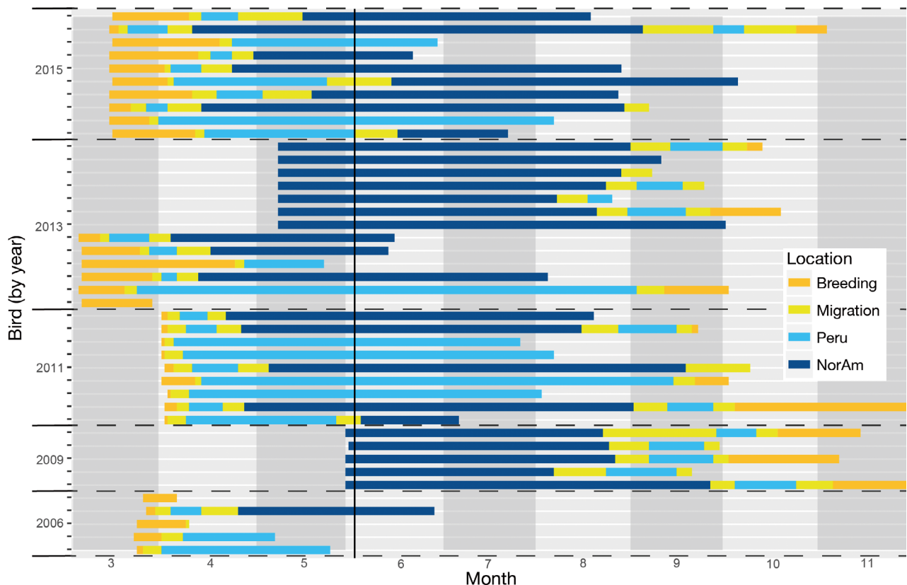
Fig. 3. Deployment plot of individual pink-footed shearwater Ardeana creatopus tracking data mapped to breeding (<32°S; orange), migratory corridor (yellow), and non-breeding-season residency (blue) areas over the year (by day of year) for all tagged birds, 2006–2015. Light blue indicates Peru and dark blue North America (NorAm). Vertical black line indicates latest known day of the year that any individual tagged in Chile migrated north from Peru to North America
